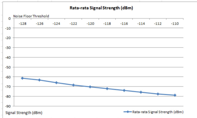
Gambar 6. Grafik Rata-rata Signal Strength Client 1, 2 & 3
