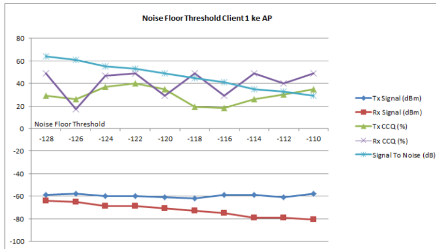
Gambar 7. Signal Strength client 1 ke AP
